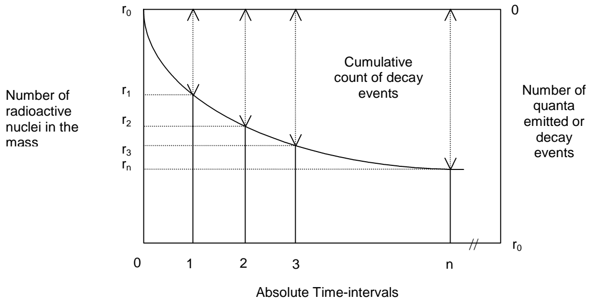
Radioactive Decay Curve Rebased on Absolute Time-intervals
